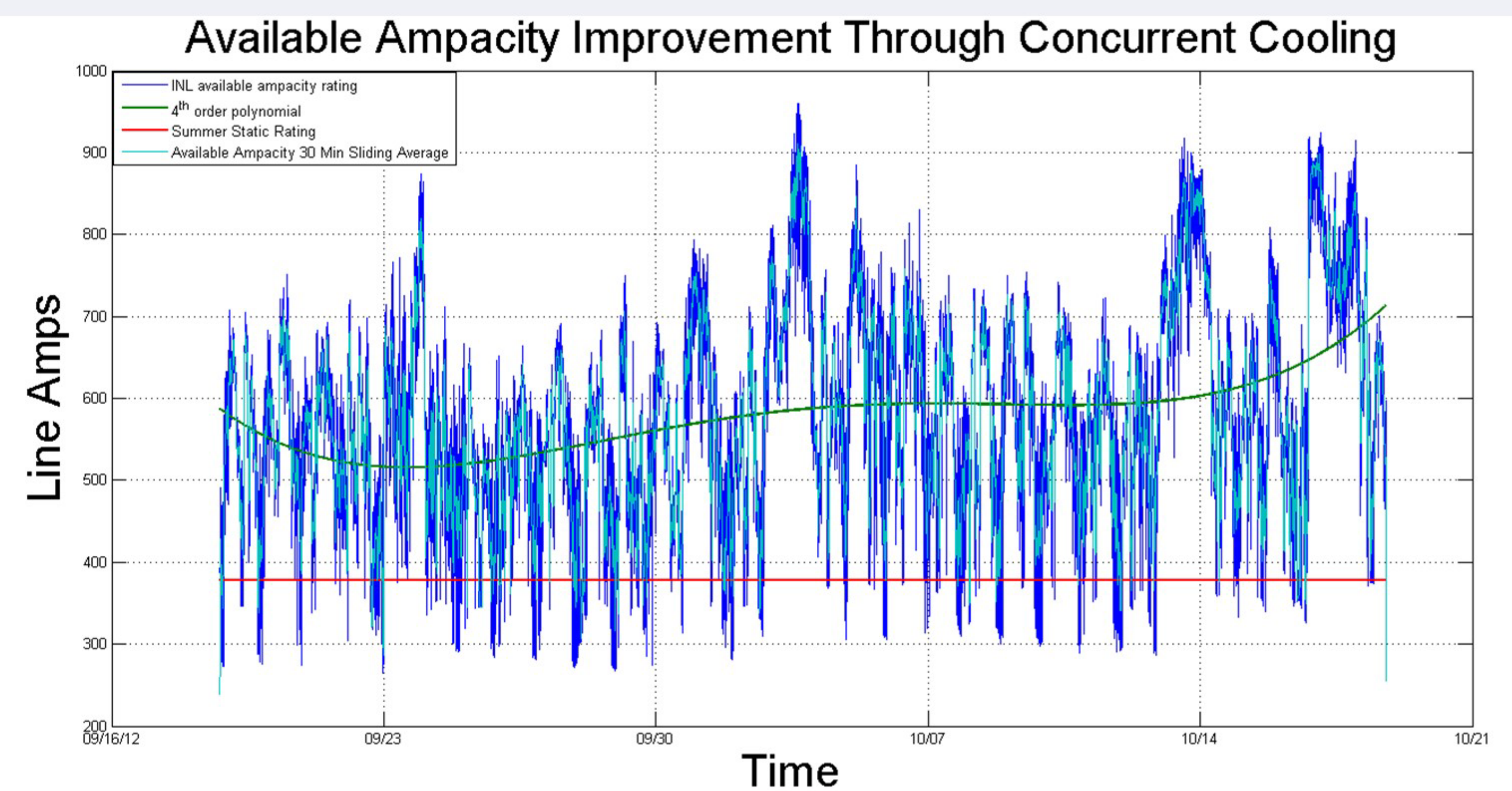
Fig. 3: Comparison of Calculated Dynamic (Blue) and Static (Red) ampacity rating
